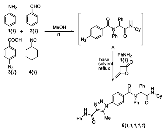
Scheme 1. One-Pot Synthesis of Triazole-Modified Peptidomimetics
